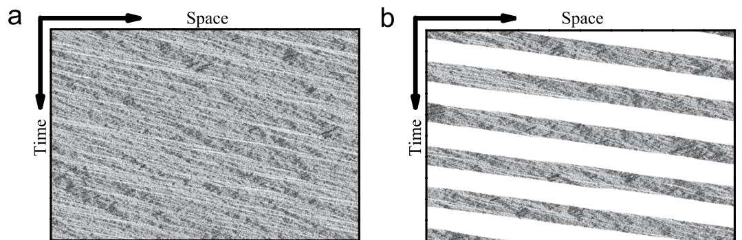
Figure 5. The spatiotemporal patterns in the bus route model. (a) Homogeneous state, the density \rho = 0.4 and p = 0.7, \lambda = 0.2 . (b) Bus bunching state, the density \rho = 0.2 and p = 0.5, \lambda = 0.02 .
